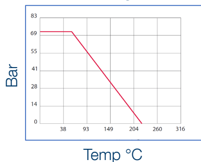
P/T Diagram
